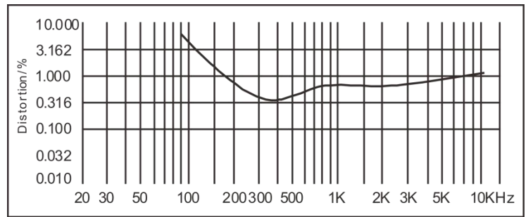
Distortion (THD < 1.5% 1W, 1m, 200Hz-10kHz)
