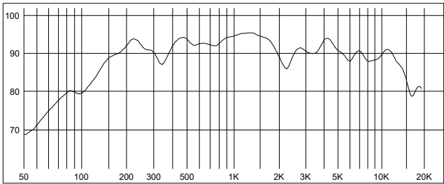
Frequency Response (dB SPL, 1W, 1m)
