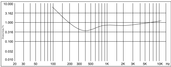
Distortion (THD<1.5% 1W, 1m, 200Hz-10kHz)
